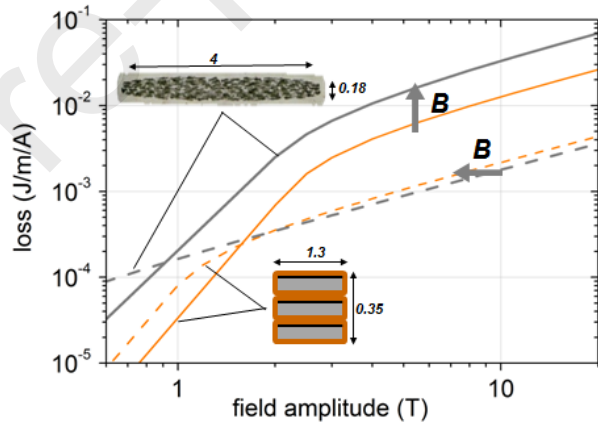
Fig. 2. Saturated loss divided by the critical current for a non-twisted stack of tapes (orange) and for a Bi-2223 tape (grey). Both parallel (dashed lines) and perpendicular (solid lines) magnetic field orientations are shown.
