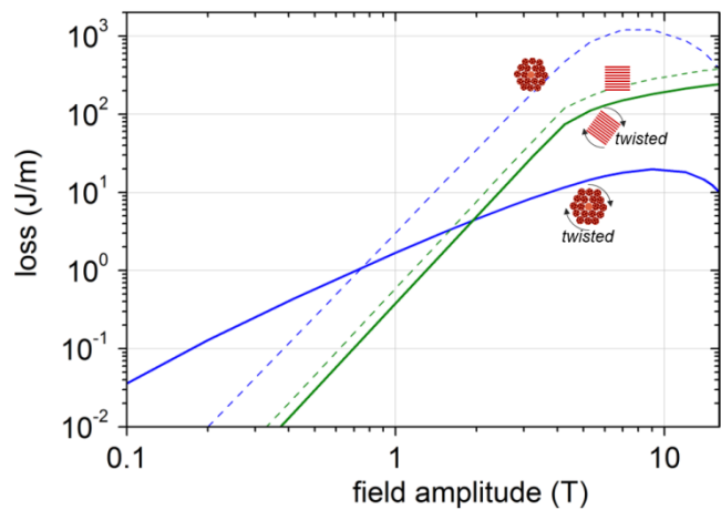
Fig. 4. Hysteretic loss (twisted, solid lines) and saturated coupling loss (non-twisted, dashed lines) for the stack of tapes (green) and the Nb 3 Sn sub-cable (blue).
