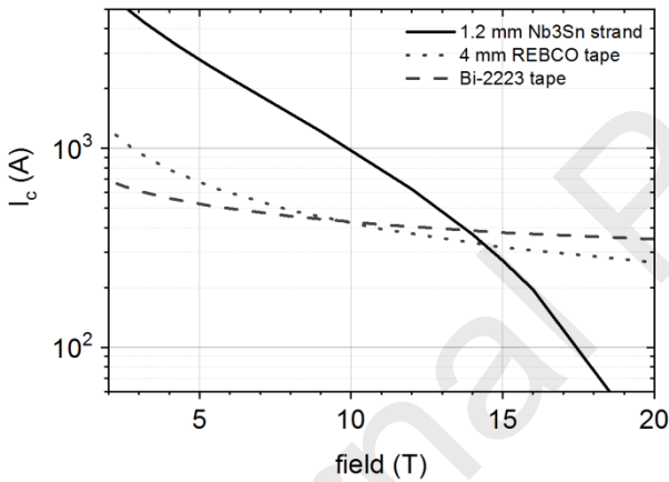
Fig. 1. Critical current versus field (at 4.2 K), for the wire and strands discussed in this paper. The curves are analytical equations representative of commercial wires and tapes.
