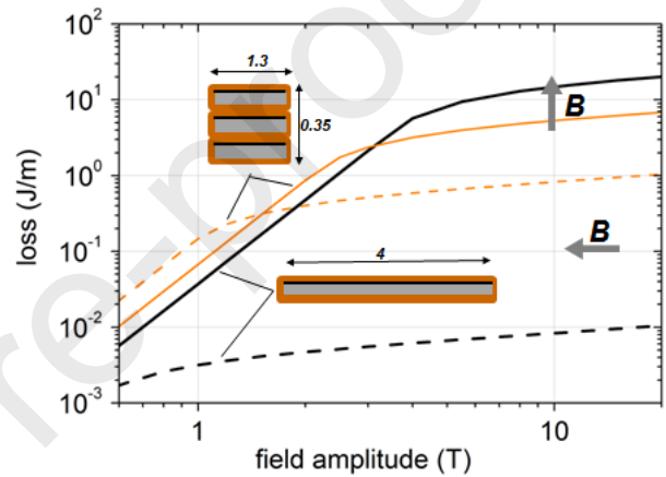
Fig. 3. Hysteretic loss (J/m) for a 4 mm wide tape (grey) and saturated loss for a non-twisted stack of three 1.3 mm wide tapes (orange). Both parallel (dashed lines) and perpendicular (solid lines) magnetic field orientations are shown.
