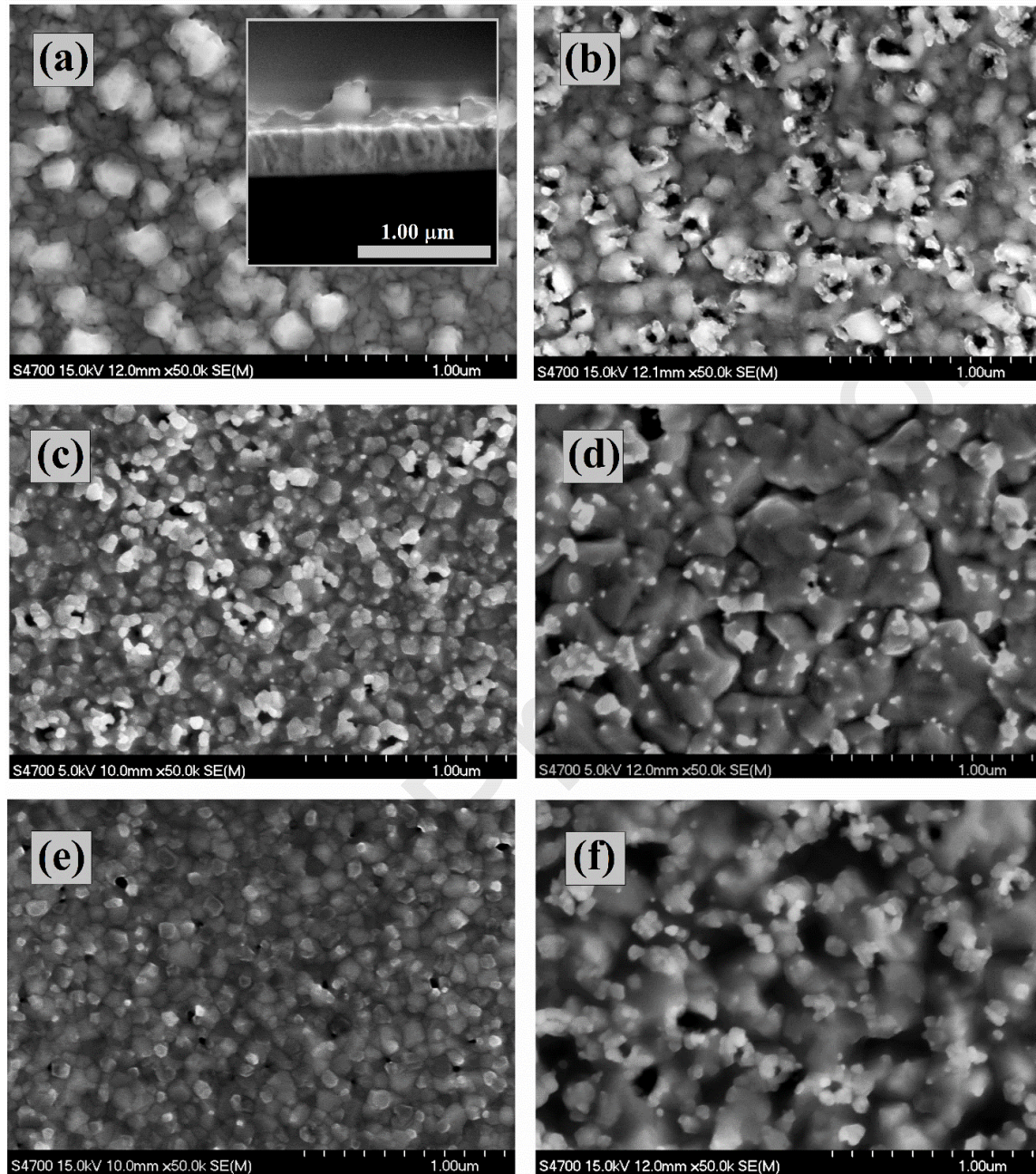
Fig. 3. SEM images of the surface of Nb 3 Sn films deposited on sapphire: (a) as-deposited, (b) annealed at 800 °C for 24 h, (c) annealed at 900 °C for 24 h, (d) annealed at 1000 °C for 24 h, (e) annealed at 1000 °C for 1 h, and (f) annealed at 1000 °C for 12 h. The inset of (a) shows the cross-section of the as-deposited film.
