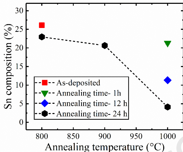
Fig. 4. Sn atomic composition of the \text{Nb}_3\text{Sn} films deposited on sapphire. The red square (■) is for the film deposited at 800 °C. The substrate heater was turned off right after deposition. The black hexagons (●) are for films deposited at 800 °C then annealed for 24 h. The blue diamonds (◆) and green triangles (▼) are for films annealed at 1000 °C for different times.
