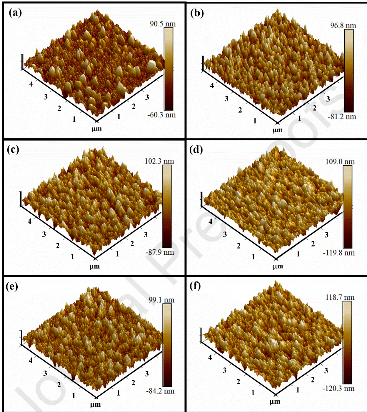
Fig. 5. AFM images of ( 5\mu\text{m} \times 5\mu\text{m} ) scan size of \text{Nb}_3\text{Sn} films on sapphire: (a) as-deposited, (b) annealed at 800 °C for 24 h, (c) annealed at 900 °C for 24 h, (d) annealed at 1000 °C for 24 h, (e) annealed at 1000 °C for 1 h, and (f) annealed at 1000 °C for 12 h.
