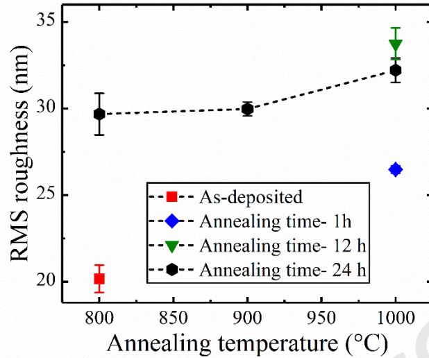
Fig. 6. RMS surface roughness of \text{Nb}_3\text{Sn} films on sapphire. The error bars represent the standard deviation of different measurements.
